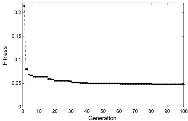
Fig. 3. Convergence of fitness function
