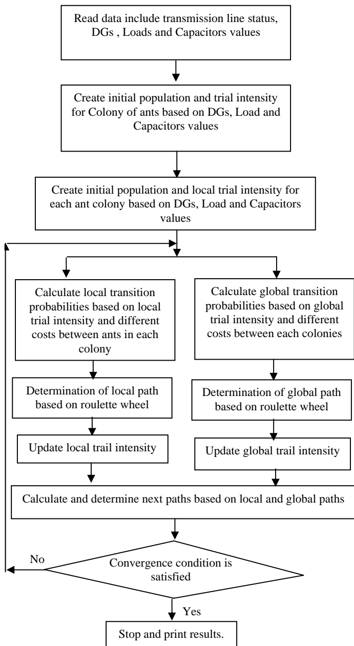
Fig. 5 Flowchart of proposed algorithm
