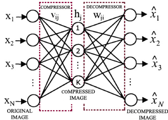
Fig. 1 Basic image compression structure using neural network
