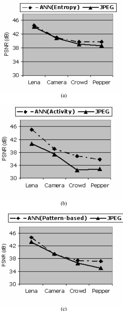
Fig. 10 The comparison of the adaptive methods with the JPEG compression standard: (a) Entropy, (b) Activity and (c) Pattern-based
