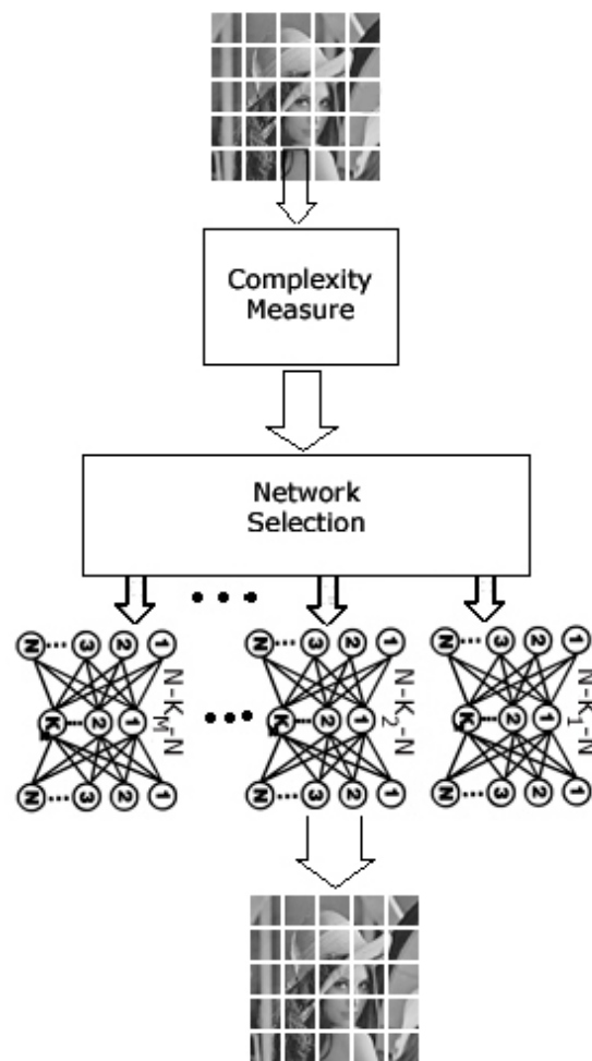
Fig. 2 Neural network-based adaptive structure for image compression
