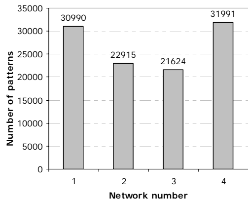
Fig. 9 The histogram of number of training blocks for 4 Activity values range for 105 images in training set. (i.e. Number of patterns= 105 \times (256 \times 256) : images size) =107520)
