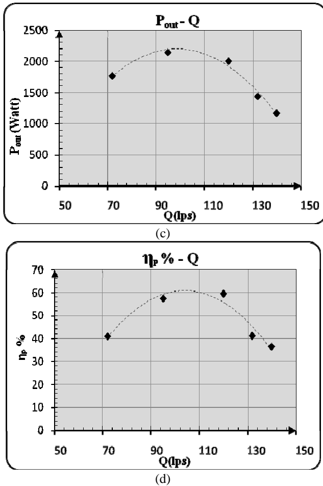
Fig. 3 Pump characteristic curves; a- Head versus flow rate, b- Input power versus flow rate, c- Output power versus flow rates, d- Efficiency versus flow rate.
