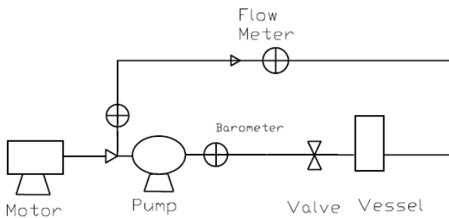
Fig. 1 Axial flow pump test region
