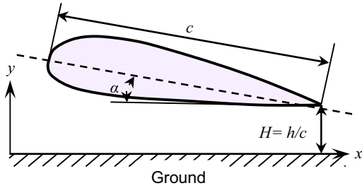
Fig. 1 Physical model and coordinate system of airfoil
