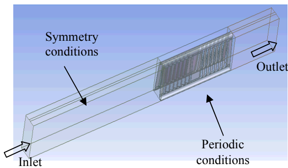
Fig. 2 Computational domain
