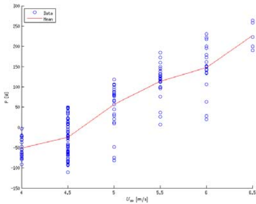
Fig. 6: Power production with respect to the wind speed for a fixed rotor angular velocity of 150 rpm
