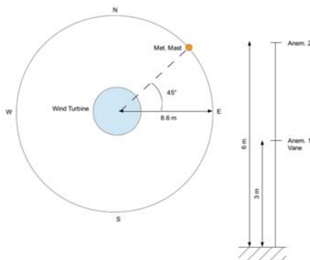
Fig. 4: Meteorological mast installation scheme
