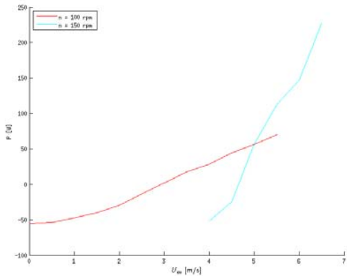
Fig. 7: Mean power production with respect to the wind speed for angular velocities of 100 and 150 rpm
