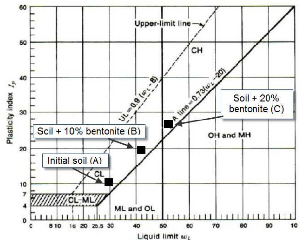
Fig. 9 Locations of three soils in plasticity chart
