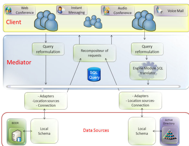
Fig. 2 Architecture of the prototype mediation
