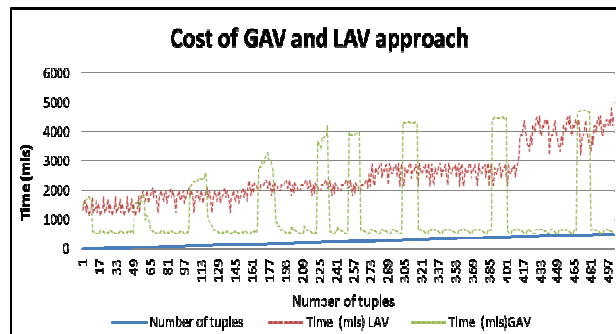
Fig. 8 Cost of GAV and LAV approach
