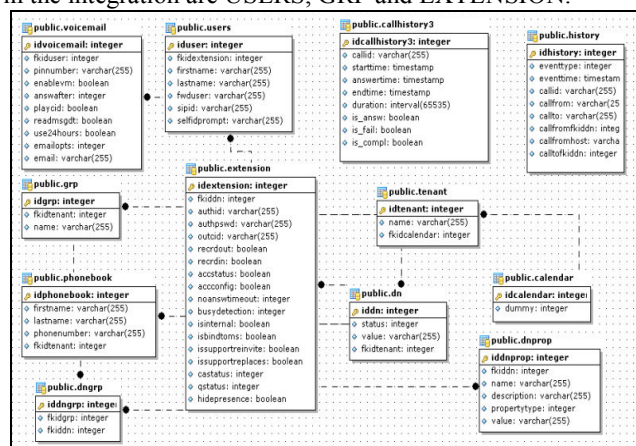
Fig. 3 Diagram of the database 3CX
