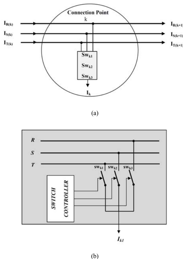
Fig. 1. (a) Distribution Feeder around point k (b) Load Switching Configuring for a load
