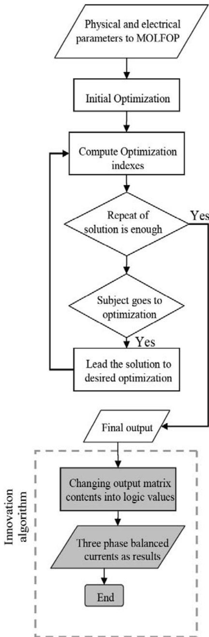
Fig. 2. The MOLFOP Algorithm for Load Balancing
