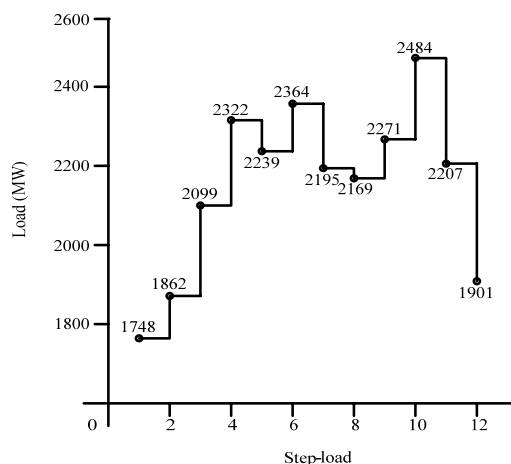
Fig. 3 Daily load patterns
