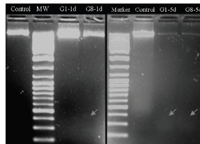
Fig. 4 Effects of gramine on DNA structures of M. aeruginosa cells. From the left to the right of the above label, cells without treatment, showing 'control', cells with 1 \text{ mg}\cdot\text{L}^{-1} of gramine treatments for 1 d, showing 'G1-1d', 8 \text{ mg}\cdot\text{L}^{-1} for 1 d, showing 'G8-1d', 1 \text{ mg}\cdot\text{L}^{-1} for 5 d, showing 'G1-5d', 8 \text{ mg}\cdot\text{L}^{-1} for 5 d, showing 'G8-5d'. DNA small fragmentation was arrowed.
