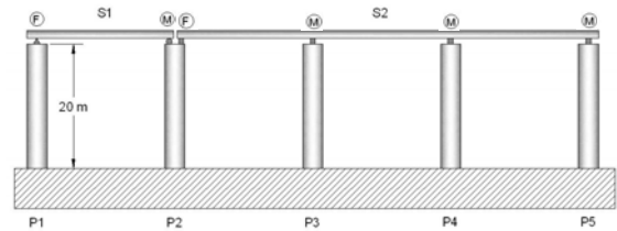
(b) Elevation view of steel bearings viaduct (SB)
