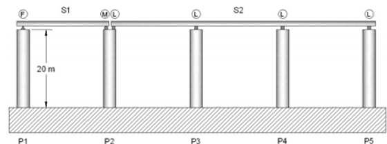
(c) Elevation view of LRB supports viaduct (LRB)
