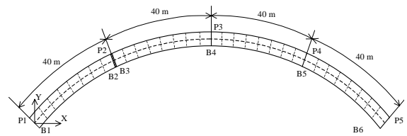
(a) Plan view of viaduct
