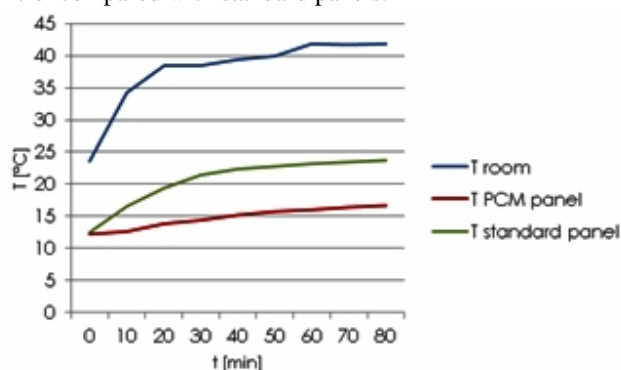
Fig. 10 Temperature variations recorded on the surface of innovative composite panels and standard panels
