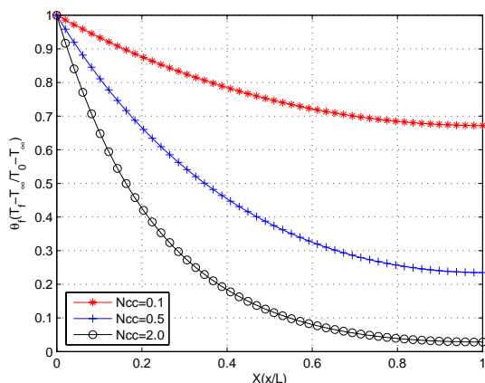
Fig. 8 Conjugate stretching sheet temperature distributions for M=0.1 ,
