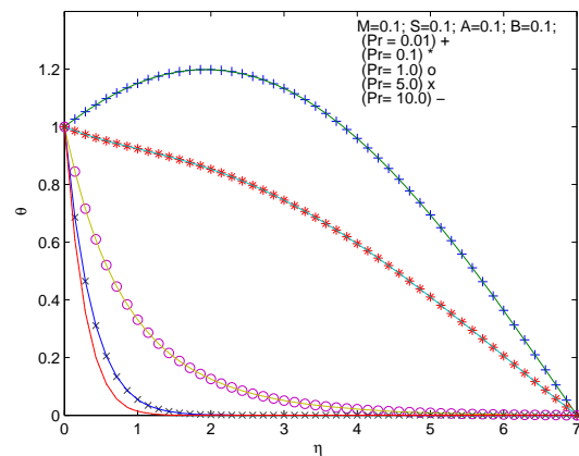
Fig. 3 dimensionless temperature profiles \theta vs. \eta as M=0.1, S=0.1, A=0.1, B=0.1 and Pr=0.01, 0.1, 1.0, 5.0, 10.0 .
