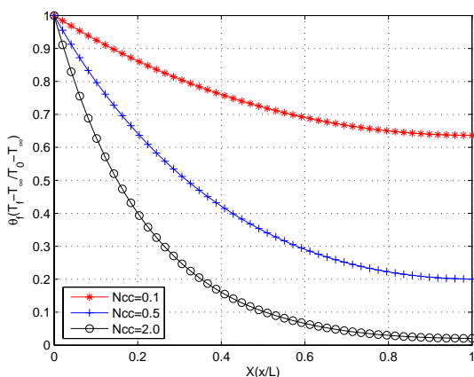
Fig. 9 Conjugate stretching sheet temperature distributions for M=0.1 ,
