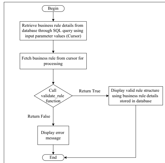
Fig. 8 check_rule procedure logic for business rule validation
