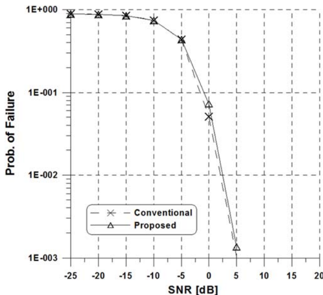
Fig. 3. Probability of failure of the conventional and proposed IFO estimator versus SNR
