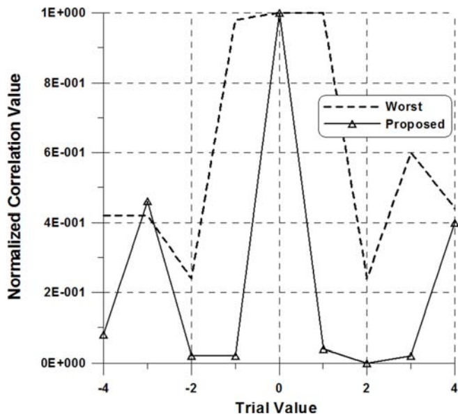
Fig. 2. Normalized correlation value of the proposed IFO estimator when \Delta_i = 0
