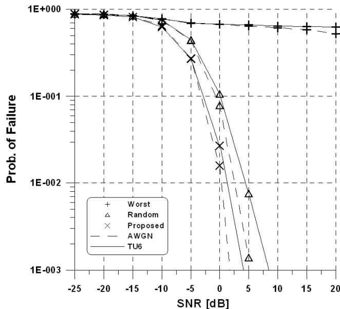
Fig. 4. Probability of failure of the proposed IFO estimator versus SNR: (1) dashed lines - AWGN (2) solid lines - TU6 channel model
