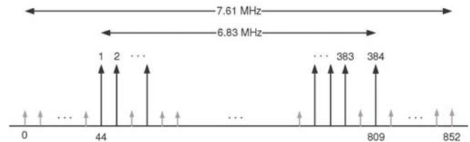
Fig. 1. The P1 symbol in the DVB-T2 system
