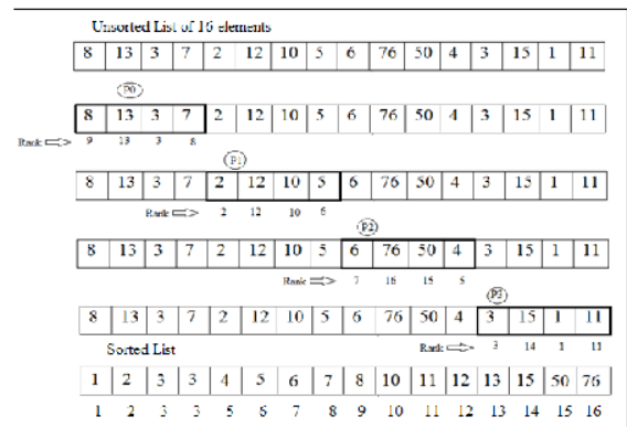
Fig. 4 Parallel Rank Sort Algorithm
