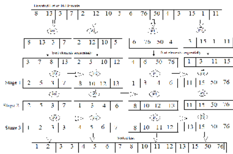
Fig. 2 Odd-Even Transposition Sort
