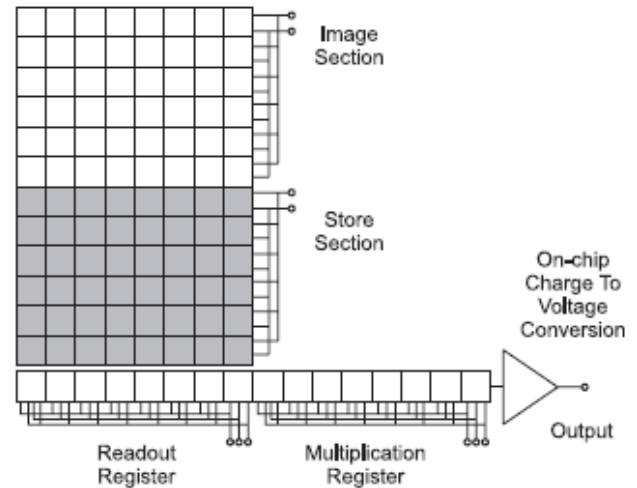
Fig. 1 EMCCD Structure
