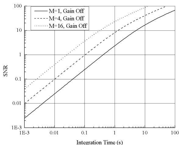
Fig. 4 Variation of the SNR versus integration time for an cooled EMCCD with different binning factors (Gain Off)
