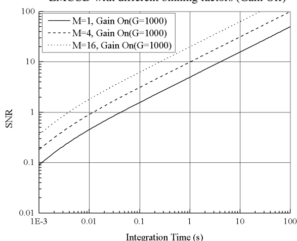
Fig. 5 Variation of the SNR versus integration time for an cooled EMCCD with different binning factors (G=1000)
