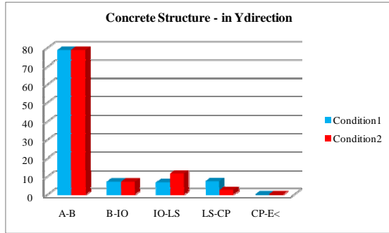
Fig. 2 (b): C1 Structure-Y direction
