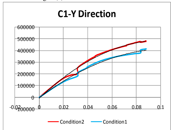
Fig. 3 (b): C1 Structure-Y direction
