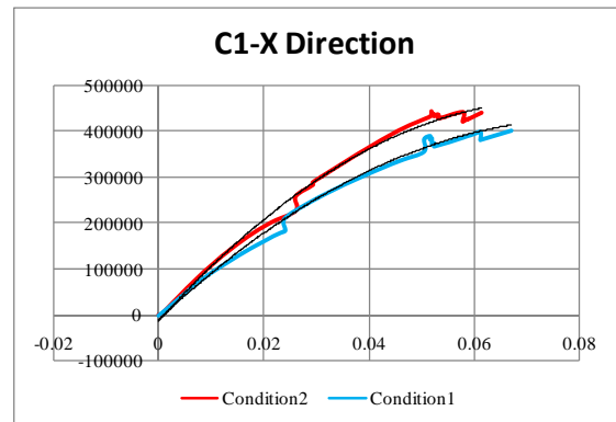
Fig. 3 (a): C1 Structure-X direction
