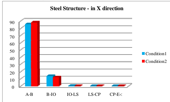
Fig. 2 (c): S1 Structure-X direction
