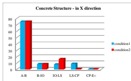
Fig. 2 (a): C1 Structure-X direction
