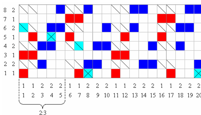
Fig. 7 Screenshot from WeaveStudio CAD/CAM software of double-layer twill weave in the warp ratio 2:3 and weft ratio 1:1
