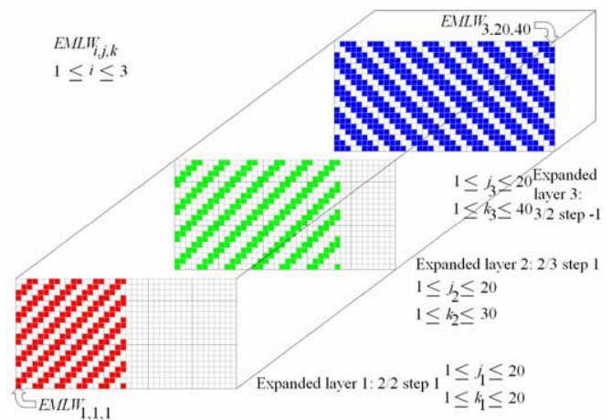
Fig.13 Adapted screenshot from WeaveStudio CAD/CAM software of expanded 2D weave assembly
