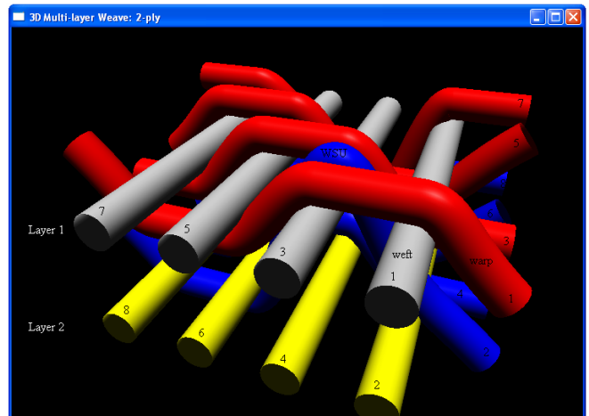
Fig. 5 Screenshot from WeaveStudio CAD/CAM software of double-layer twill weave geometry and warp stitch up layer binding
