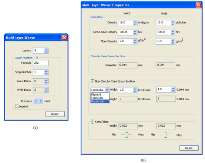
Fig. 11 Screenshot from WeaveStudio CAD/CAM software of (a) multi-layer weave specification and (b) multi-layer weave properties
