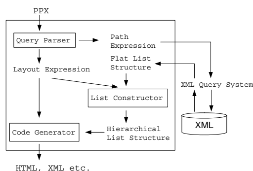
Fig. 7. System architecture
