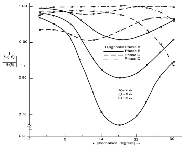
Fig. 3 Back-of-core saturation effects on position signal
