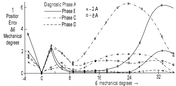
Fig. 9 Position errors due to back-of-core saturation
