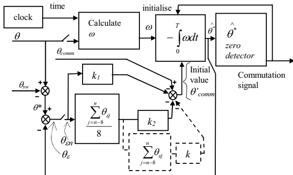
Fig. 8 Block diagram of position extrapolation process
