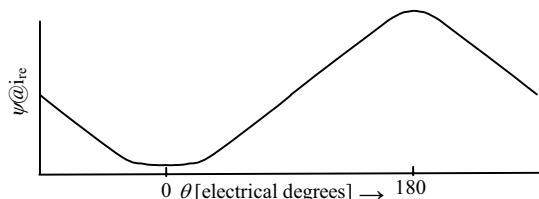
Fig. 5 Diagnostic flux-linkage at a given current
