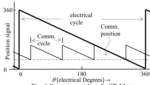
Fig. 6 Operation cycles of a SR Motor
