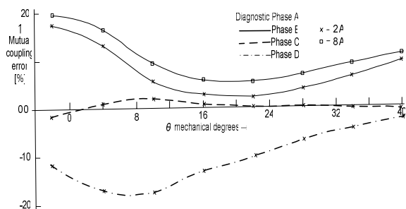
Fig. 10 Error due mutual coupling between phases
