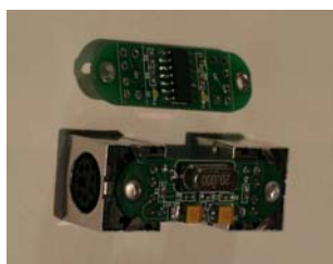
Fig. 5 Implemented and reprogrammed security hardware for PS/2 keyboard as an example. USB keyboard is not considerable for a secure keyboard because the USB host controller has no disposable interface between the host and the target device and it is adapted to the PS/2 interface through a combo converter
