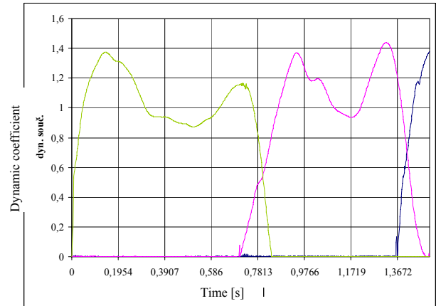
Fig. 4 Force record from gauge configuration – variant 1
