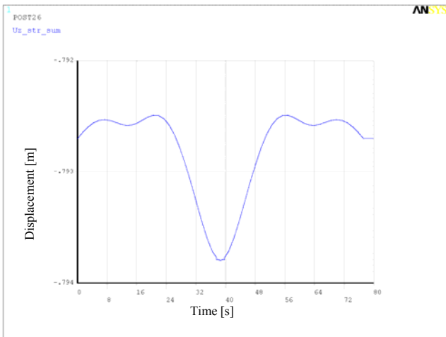
Fig. 33 Vertical displacement U_z , mid span, Variant No. 10
