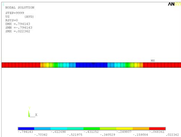
Fig. 22 Maximal envelope U_z total, Variant No. 9
