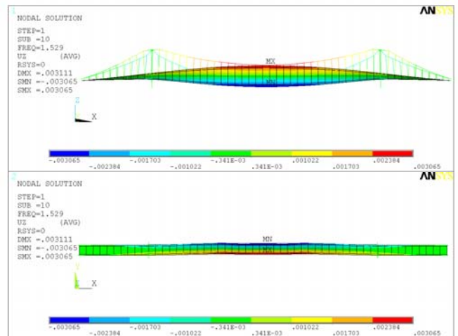
Fig. 13 Eigen shape according to f = 1.529 \text{ Hz}
