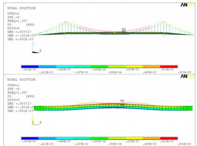
Fig. 12 Eigen shape according to f = 1.367 \text{ Hz}
