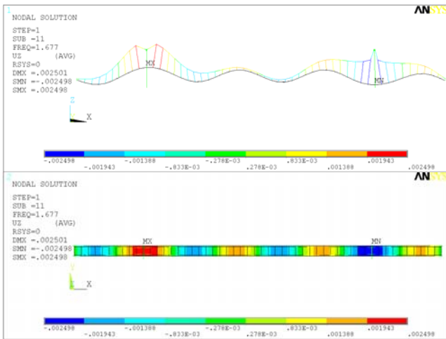
Fig. 14 Eigen shape according to f = 1.677 Hz
