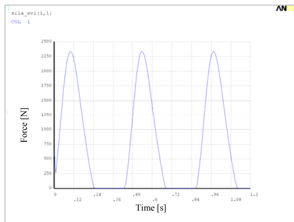
Fig. 21 Vertical force time record for running
