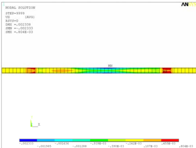
Fig. 28 Maximal envelope U_z dynamic, Variant No. 3 – torsional
