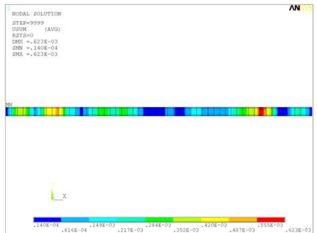
Fig. 27 Maximal envelope U_{SUM} , Variant No. 9
