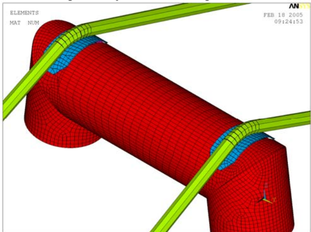
Fig. 11 Computational model – detail view
