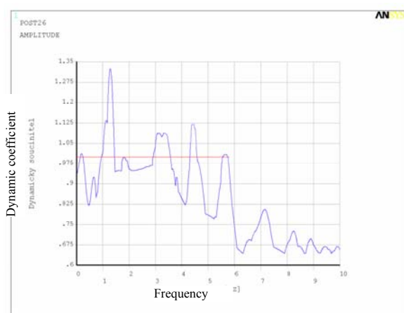
Fig. 8 Force-frequency record
