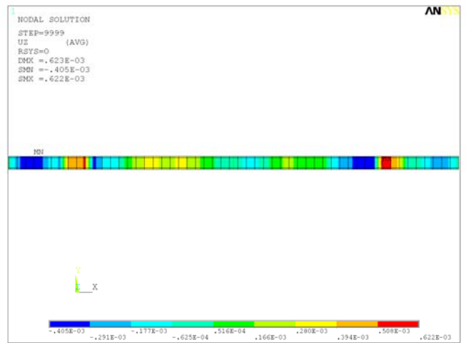
Fig. 26 Maximal envelope U_z dynamic, Variant No. 9
