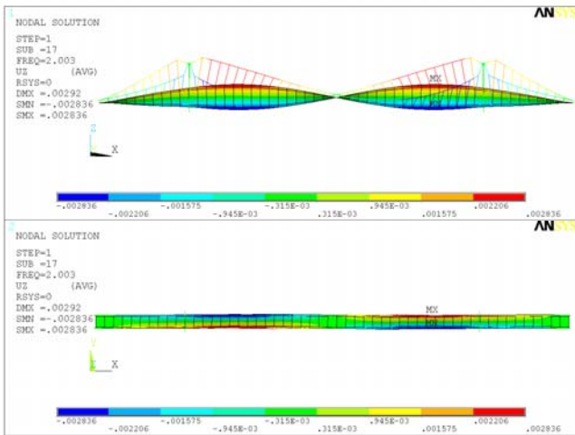
Fig. 16 Eigen shape according to f = 2.003 Hz
