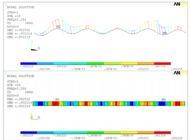
Fig. 17 Eigen shape according to f = 2.286 Hz
