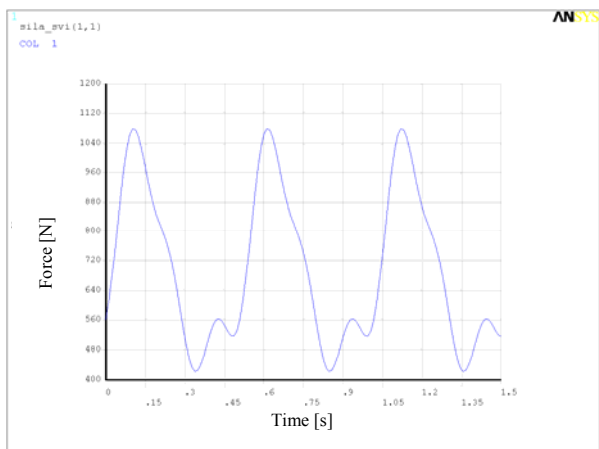
Fig. 18 Vertical force time record
