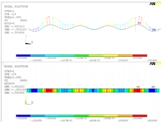
Fig. 15 Eigen shape according to f = 1.965 Hz
