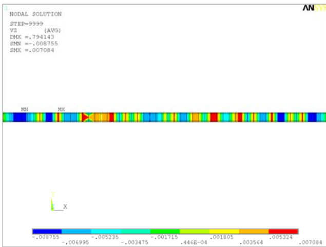
Fig. 23 Maximal envelope V_z , Variant No. 9
