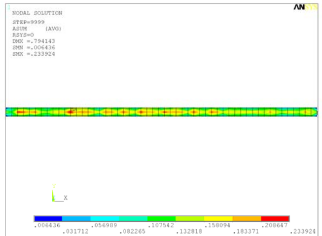
Fig. 25 Maximal envelope A_{SUM} , Variant No. 9
