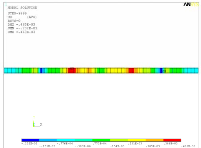
Fig. 31 Maximal envelope U_z dynamic, Variant No. 7
