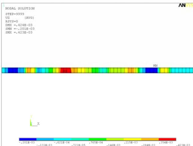
Fig. 30 Maximal envelope U_z dynamic, Variant No. 2
