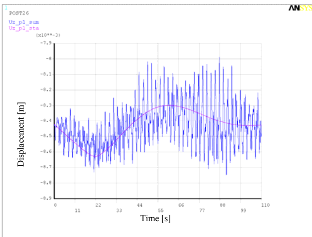
Fig. 34 Total and static vertical displacement U_z , near pylon p_1 , Variant No. 3
