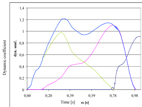
Fig. 7 Force record from gauge configuration – variant 2
