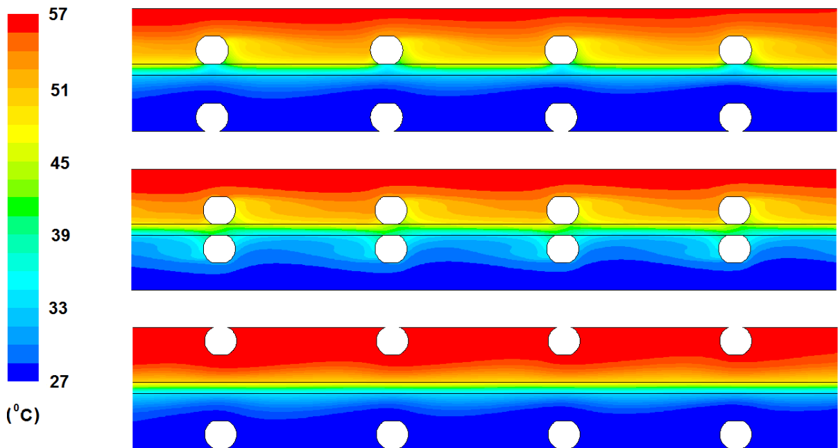
Fig. 2 Temperature profiles in spacer-filled channels
