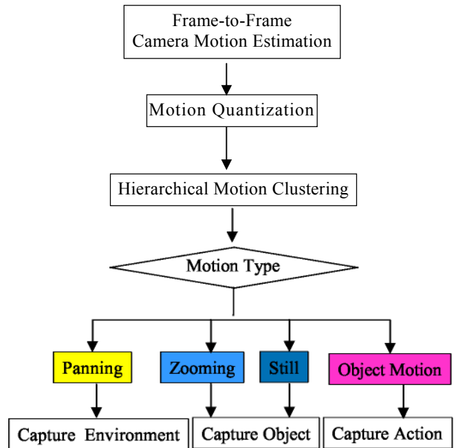
Fig. 2 Flow diagram of video motion mining algorithm
