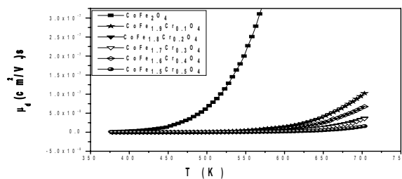
Fig.4 Graph between drift mobility ( \mu_d ) and temperature for \text{CoFe}_{2-x}\text{Cr}_x\text{O}_4 where x=0.0, 0.1, 0.2, 0.3, 0.4 and 0.5
