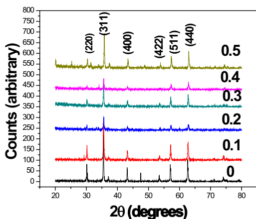
Fig. 1 XRD patterns for \text{CoFe}_{2-x}\text{Cr}_x\text{O}_4 where x=0.0, 0.1, 0.2, 0.3, 0.4, 0.5 (sintered)
