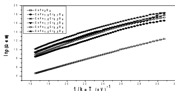
Fig. 3 Graph between resistivity ( \ln\rho ) and temperature for \text{CoFe}_{2-x}\text{Cr}_x\text{O}_4 where x=0.0, 0.1, 0.2, 0.3, 0.4, 0.5
