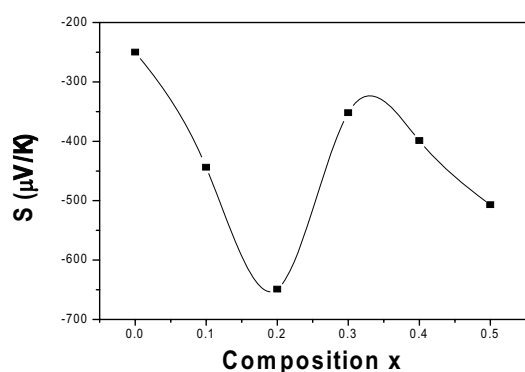
Fig. 5 Variation of Seebeck coefficient 'S' with composition \text{CoFe}_{2-x}\text{Cr}_x\text{O}_4 where x=0-0.5
