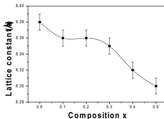
Fig. 2 Variation of lattice constant ' a ' with composition x
