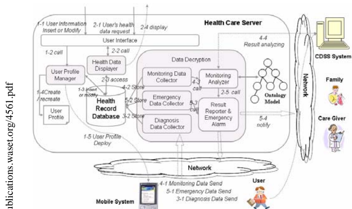
Fig. 3 Healthcare server architecture
