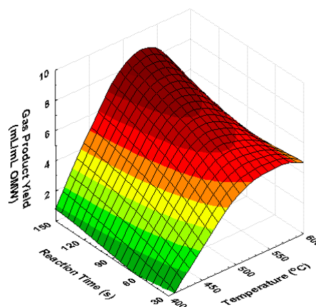
Fig. 4 The change of gas product yield with temperature and reaction time, for Ni/Al 2 O 3 catalyst
