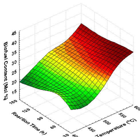
Fig. 8 The change of total biofuel content with temperature and reaction time, for Ni/Al 2 O 3 catalyst
