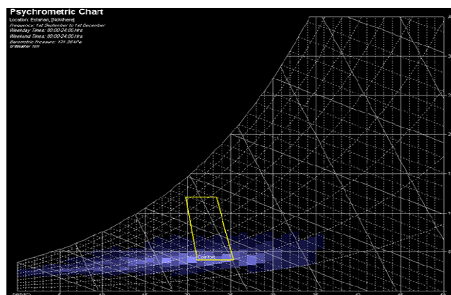
Fig. 4 Psychrometric chart, Autumn
