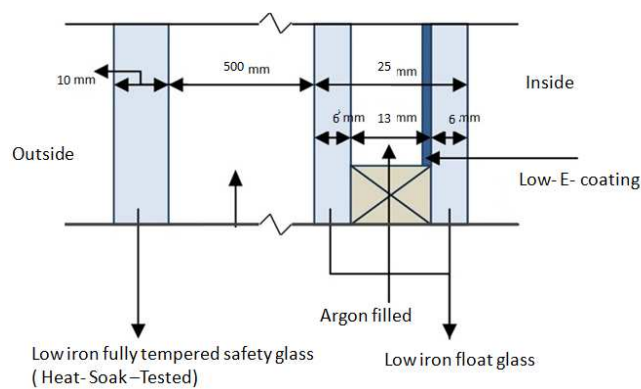
Fig. 5 Cross-Section of Suggested System
