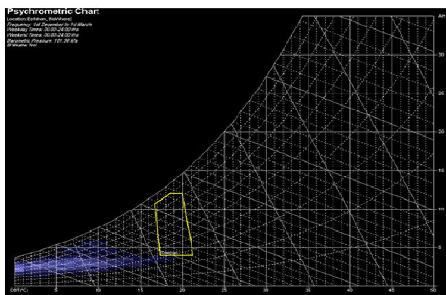
Fig. 1 Psychrometric chart, Winter
