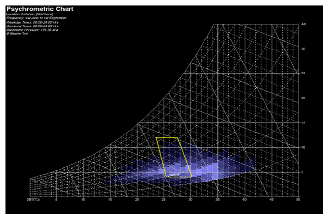
Fig. 3 Psychrometric chart, Summer
