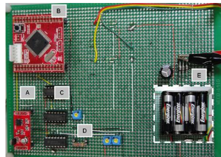
Fig. 5 Photograph of VLC Device1 as a mobile terminal
