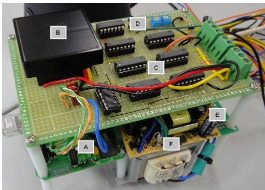
Fig. 3 Photograph of VLC Device 0
