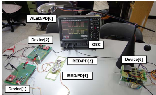
Fig. 7 Experimental setup for optical wireless sensor network
