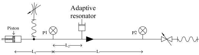
Fig. 5 Principle of the experimental device
