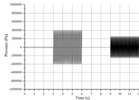
Fig. 11 Pressure at the 1.03 m point in the main pipe which also has a Helmholtz resonator at the same point
