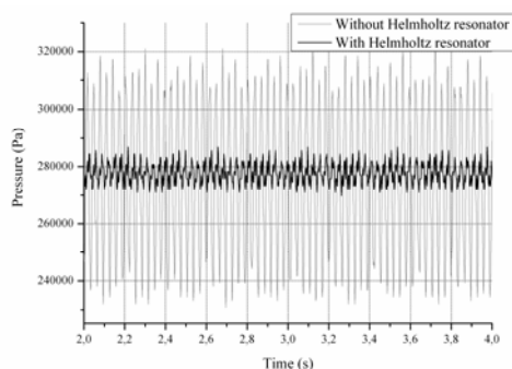
Fig. 15 Measured pressures at pressure sensor P_2
