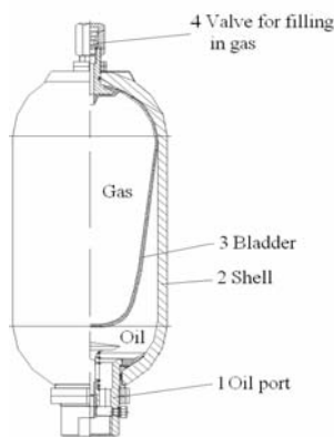
Fig. 1 Cross-section of a pressure accumulator
