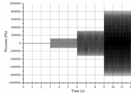
Fig. 10 Pressure at the 1.03 m point in the main pipe
