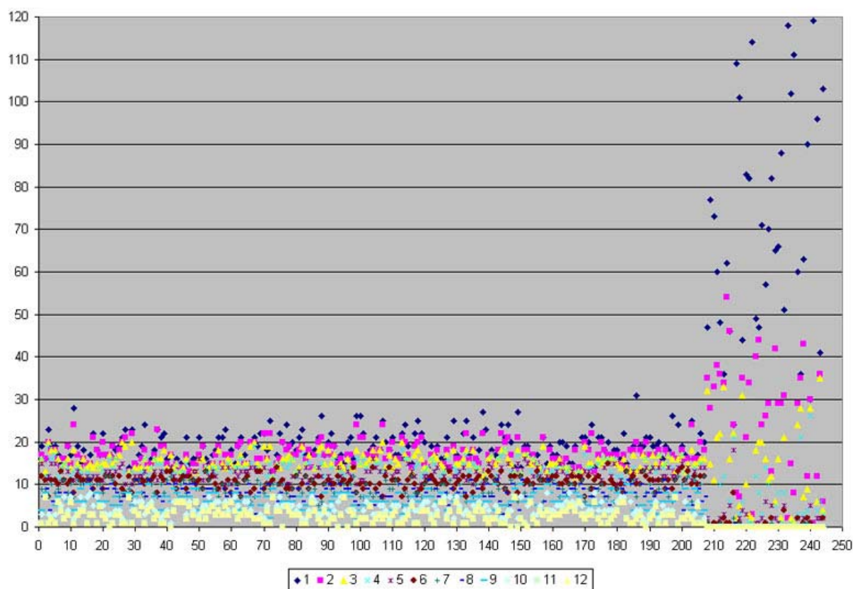
Fig. 3 Generated 85% IUD sample
