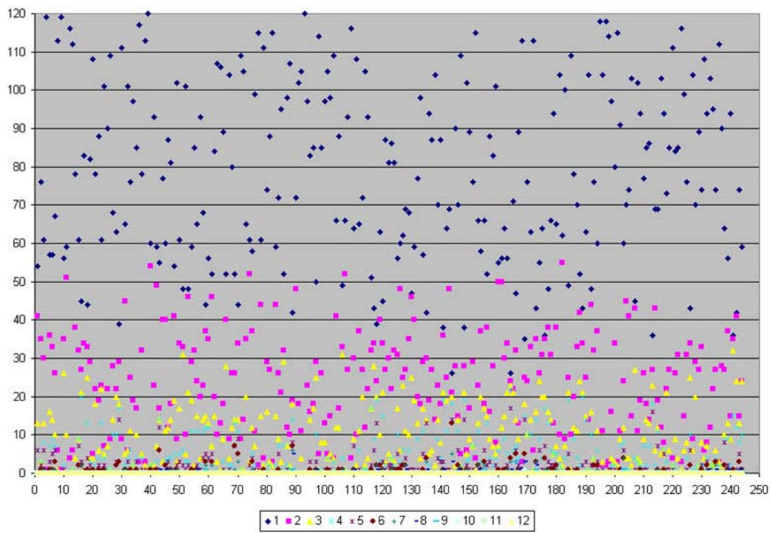
Fig. 2 Generated sample by digressive type
