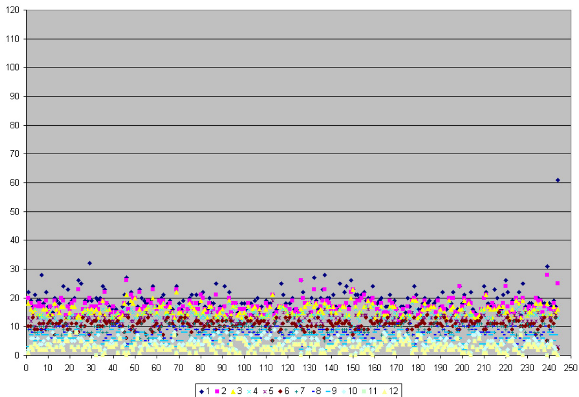
Fig. 1 Generated sample by IUD (245 strategies)
