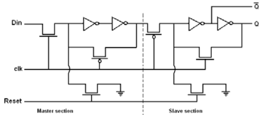
Fig. 4 D Flip Flop using pass transistors
