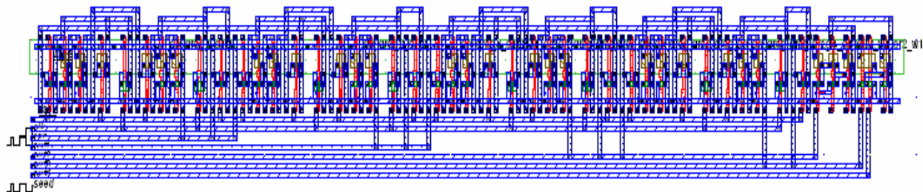
Fig. 8 Layout of LFSR in microwind
