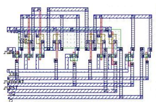
Fig. 7 Layout of D Flip Flop using Pass transistor
