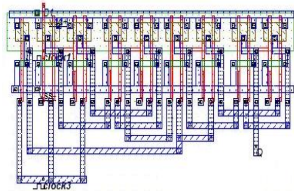
Fig. 5 Layout of D Flip Flop using NAND gate
