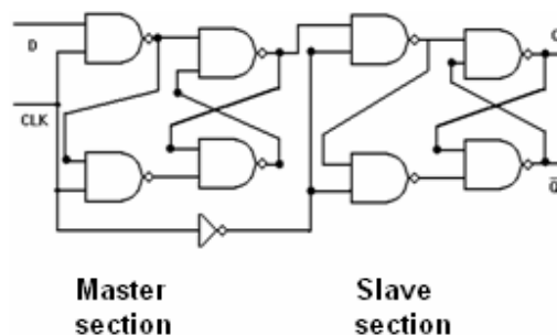
Fig. 2 D Flip Flop using NAND gates
