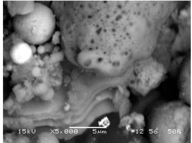
Fig. 6(a) Scanning electron micrograph of (15FA+85O/B)+2L
