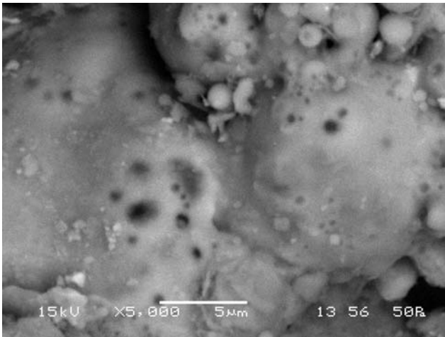
Fig. 6(e) Scanning electron micrograph of (20FA+80O/B)+2L
