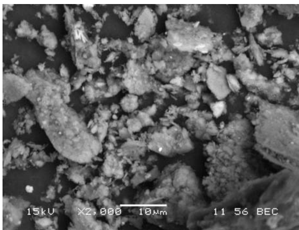
Fig. 1 Scanning electron micrograph of mine overburden
