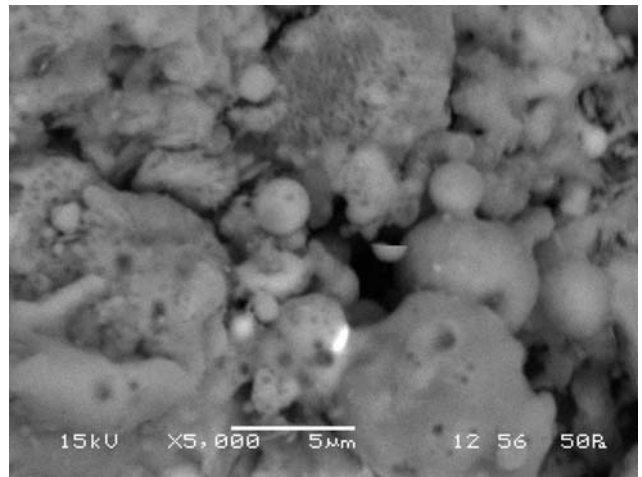
Fig. 6(b) Scanning electron micrograph of (15FA+85O/B)+3L
