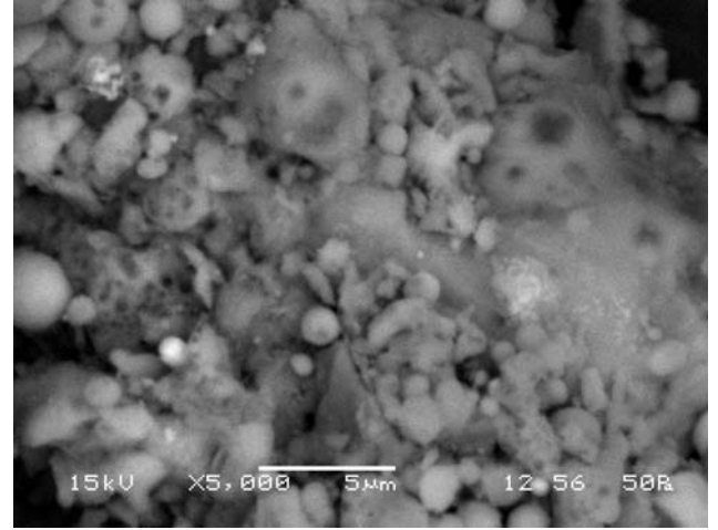
Fig. 6(o) Scanning electron micrograph of (30FA+70O/B)+6L
