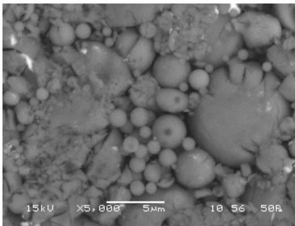
Fig. 2 Scanning electron micrograph of fly ash
