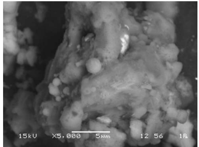
Fig. 6(h) Scanning electron micrograph of (20FA+80O/B)+9L
