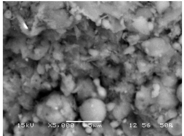
Fig. 6(m) Scanning electron micrograph of (30FA+70O/B)+2L
