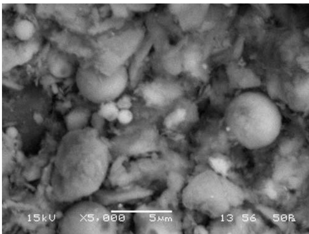
Fig. 6(f) Scanning electron micrograph of (20FA+80O/B)+3L
