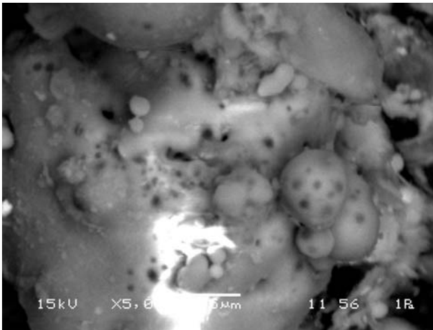
Fig. 6(j) Scanning electron micrograph of (25FA+75O/B)+3L
