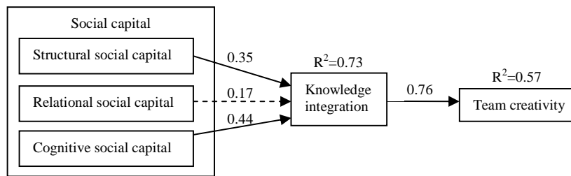
Fig. 2 PLS results for the proposed research model
