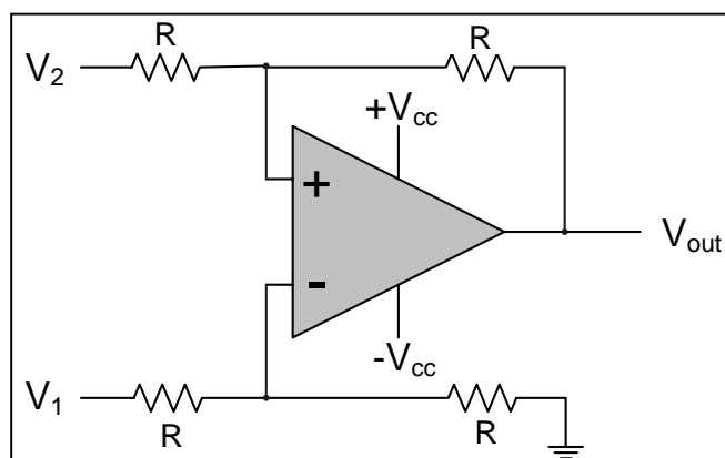
Fig.6 Differential Amplifier Interface Unit
