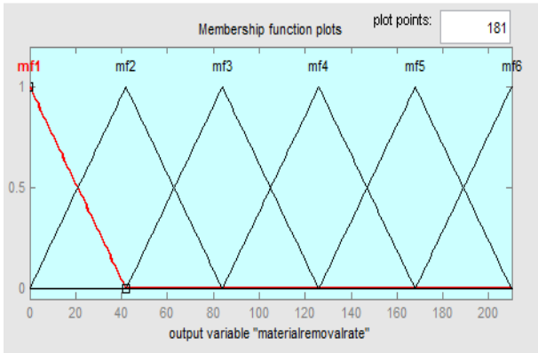
Fig. 5 Membership Functions for Output Parameter (MRR)
