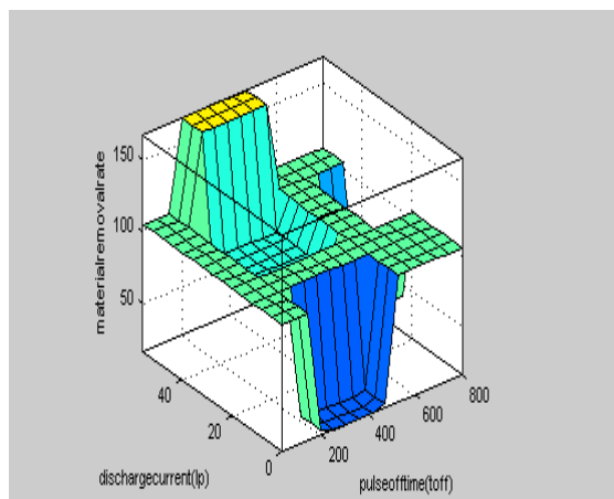
Fig. 8 Control surfaces of Fuzzy model
