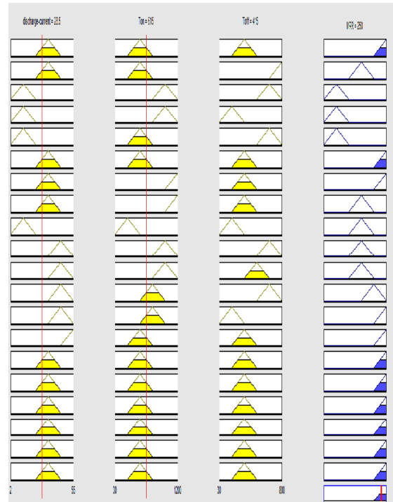
Fig. 7 Rule Viewer of Fuzzy Model (Response: MRR)
