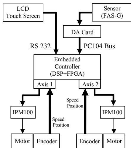
Fig. 2 Control Architecture
