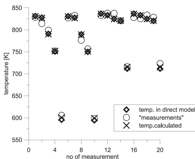
Fig. 3. The temperature values at sensor locations obtained in the iteration procedure.
