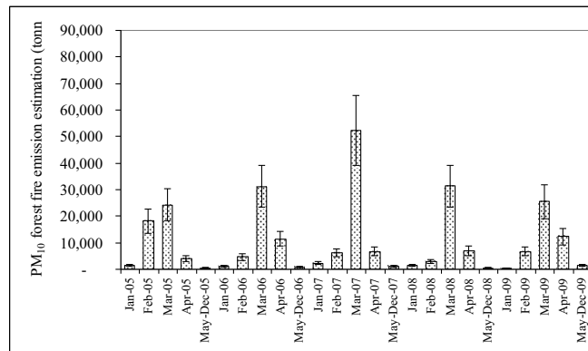
Fig.11 Monthly temporal distributions of PM 10 estimation during 2005-2009
