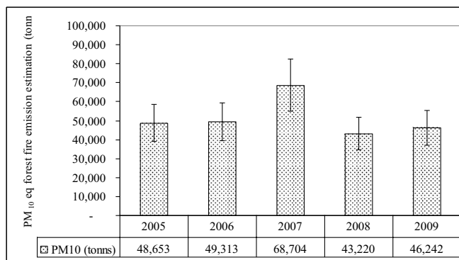
Fig. 9 Annually PM 10 estimation during 2005-2009
