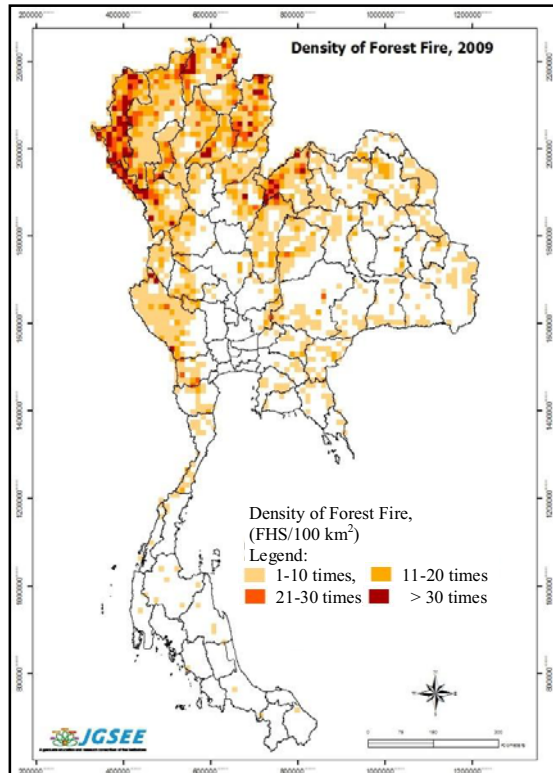
Fig. 7 Annually spatial distribution of forest fire hotspots in 2009
