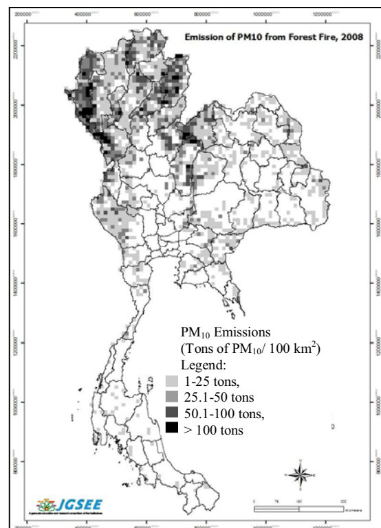
Fig.15 Spatial distribution of PM 10 from forest fire in 2008
