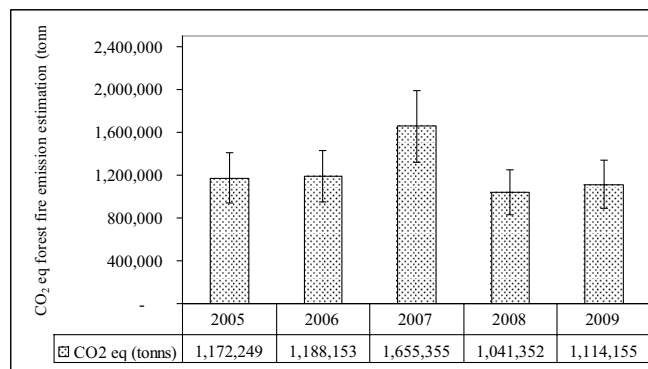
Fig. 8 Annually CO 2 eq emission estimation during 2005-2009
