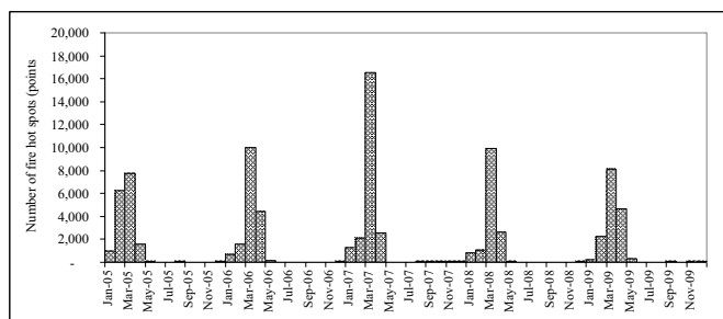
Fig. 2 Monthly distribution of fire hotspots during 2005 to 2009
