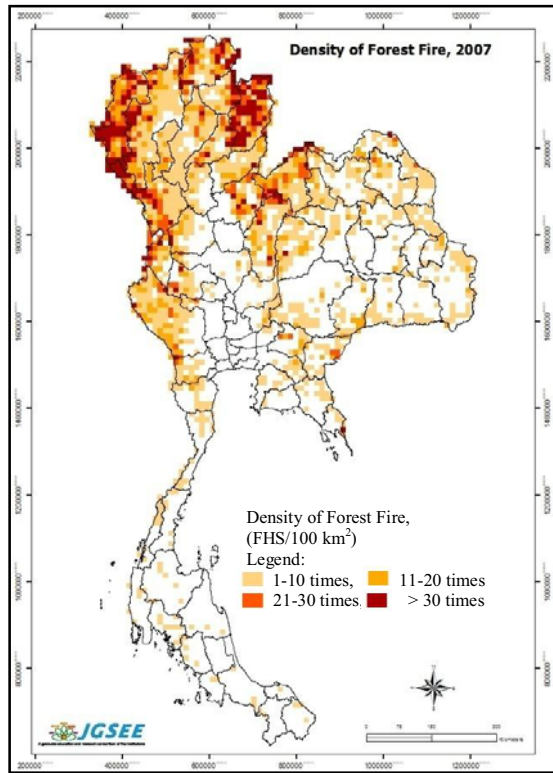
Fig. 5 Annually spatial distribution of forest fire hotspots in 2007
