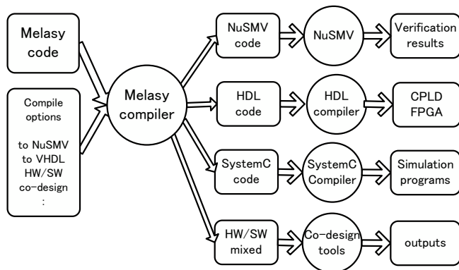
Fig. 1. The relationship of the Melasy compiler to various HDLs and the model checker.
