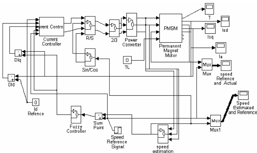
Fig. 2 The drive system with MDOFF controller and based on speed estimation
