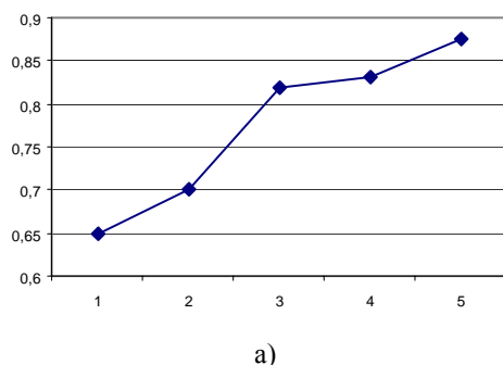
Fig. 3 Dependence of recognition probability on the size of training set by using the following parameters: a) bipartite conjugation; b) conjugation with a space stretched on the vectors from a class
