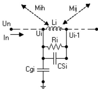
Fig.5 Equivalent circuit of the transformer winding
