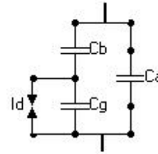
Fig.6. Three-capacitance model of PD
