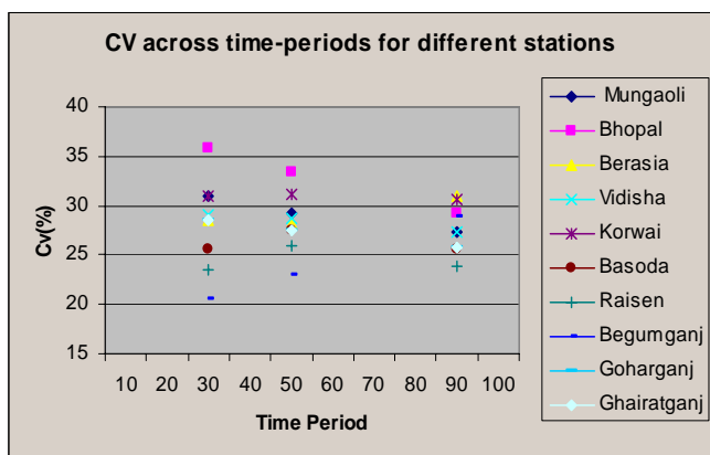
Fig. 6 (b) Temporal variation in coefficient of rainfall
