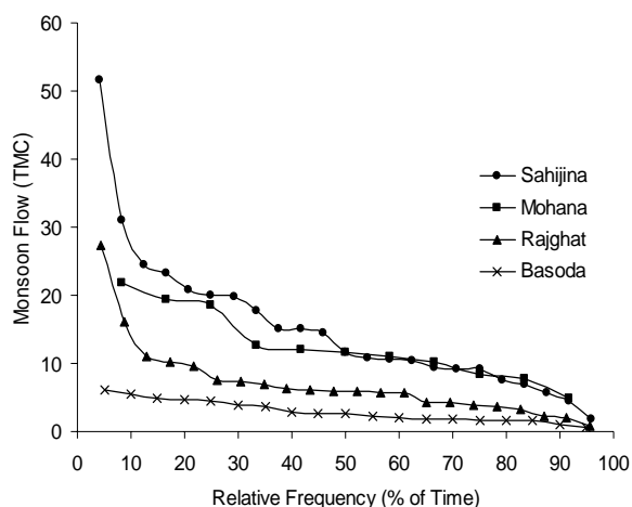
Fig. 3: Flow duration curve (1971-95)
