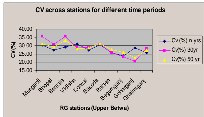
Fig. 6 (a) Spatial variation in coefficient of rainfall
