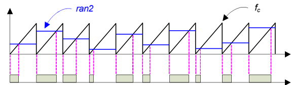
Fig. 3 The procedure of RPP generation
