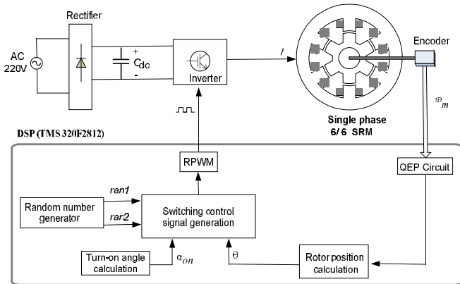
Fig. 4 Block diagram of SRM drive system.
