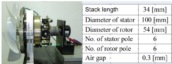
Fig. 5 Single-phase 6/6 SRM for experimentation
