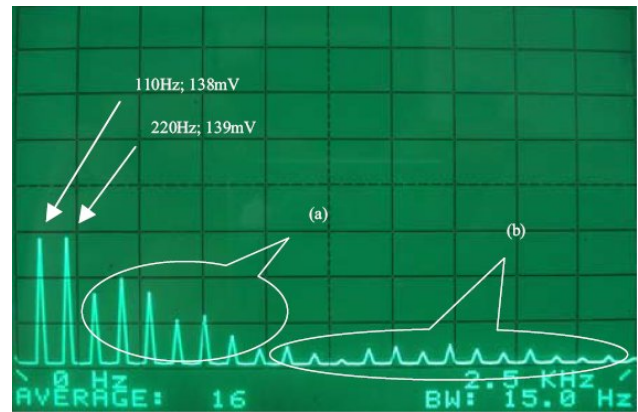
a) Conventional method with chopping mode
