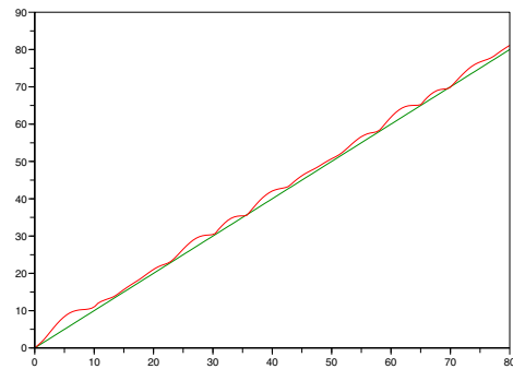
Fig. 6. Solutions (bold curves) over Dom = [0, 80] computed by the fixed point method for y'(x) = \sin(y^{-1}(x)) + 1 (top) and y'(x) = \sin(y^{-1}(x)) \cdot \cos(0.1 \cdot y^{-1}(x)) + 1 (bottom) both with initial boundary value y(0) = 0 and initialization function y(x) = x (thin curves).
