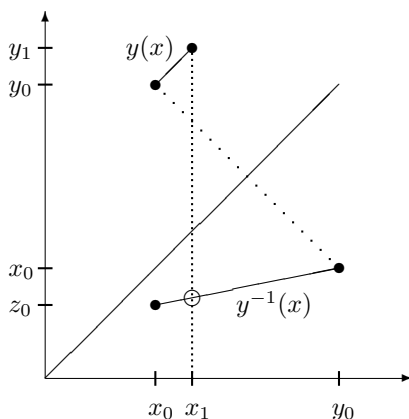
Fig. 8. Initial linear segments of the solution function and its inverse with extra specification of the initial value z_0 of the inverse function. This allows to approximate the slope of the solution function at x_1 because y^{-1}(x_1) is now approximately given.
