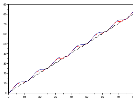
Fig. 10. Solution (bold curve, partially occluded) over Dom = [0, 80] for y'(x) = \sin(y^{-1}(x)) + 1 with initial boundary value y(0) = 0 as in figure 6 (left). Linearly induced approximating functions y_{lin}(x) = x - 2 \cdot \cos(0.5x) + 2 for \alpha = 0.5 (bold curve, same frequency and "mostly" above the solution) and y_{lin}(x) = x - 0.5 \cdot \cos(2x) - 0.5 for \alpha = 2 (thin, high frequency curve).
