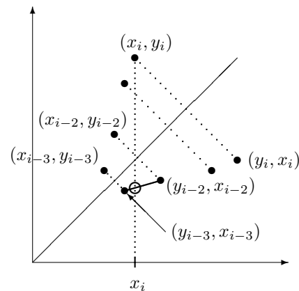
Fig. 3. Points on the function and on the inverse function with correspondences (slanted dotted lines). The value of the inverse function at support point x_i is, in this case, linearly interpolated from the values y_{i-3} and y_{i-2} so that j = i - 3 .
