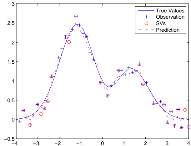
Fig. 3. Regression results of R.K
