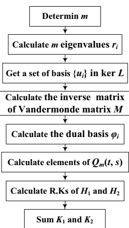
Fig. 1. Flow chart of the algorithm for the computation of reproducing kernel in W_2^m[a, b]
