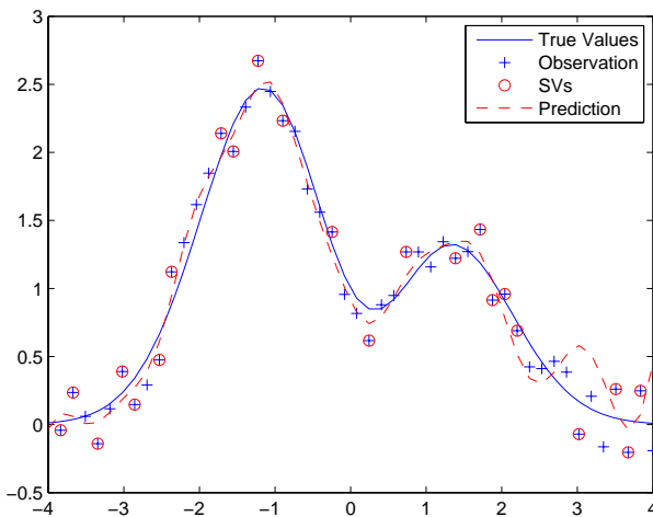
Fig. 2. Regression results of RBF
